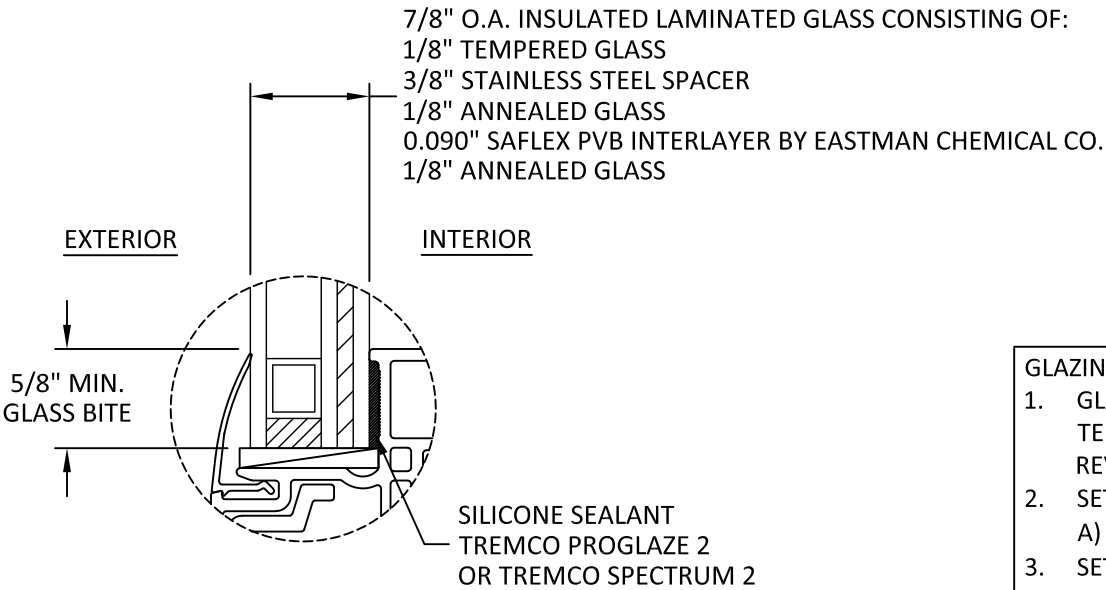
GLAZING DETAIL 1
